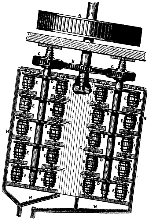
Fig. 133. Amalgamation Barrels. A is the moving wheel; B is another wheel, with 106 teeth on the axle of A ; C, C are smaller cog wheels, working to correspond with B , and each of the axes on which they are placed gives motion by means of cog wheels marked D , to a number of amalgamating casks marked E , which are all provided with a half-circular piece of iron marked F , used in conjunction with a screw, to secure the opening of the cask after the materials are put in; G, G, G, G , are also screws, the purpose of which is to enable the workmen to move any of the casks from the contact of the teeth of the wheels marked D , so that it may be worked at without stopping the movements of the other casks; H, H, H, H , indicate the iron gutter which serves to convey the mercury into any one of the casks at pleasure; they are composed of several pieces, which can be moved in any direction. In general there are 20 casks in a set, each of which contains about 300 lbs., or 30 gallons of water, and about 1000 lbs. of the decomposed mineral and pieces of scrap or forged iron. The casks are fastened up and rotated for about an hour; 500 lbs. of mercury are then put into each cask, and it is firmly closed. The machinery is so regulated as to permit the casks to turn round about fifteen or twenty times in a minute. Every four hours the amalgamation is examined, and in about sixteen hours the operation is completed.
